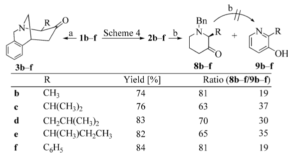
Scheme 5. (a) CAN, CH 3 CN/H 2 O (4:1), 0 °C, 30 min; (b) H 2 , 20% Pd(OH) 2 /C, AcOEt, 20 °C.
