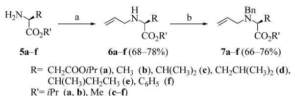
Scheme 1. (a) Allyl bromide, Li(OH)·H 2 O, MS 4 Å, DMF, 20 °C; (b) benzyl bromide, K 2 CO 3 , DMF, 20 °C.
