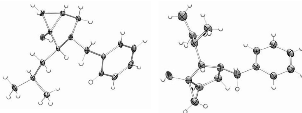
Figure 2. ORTEP plot of X-ray crystal structure of trans - 1d and cis - 1e .
